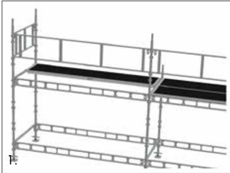
1. Install 1x600 Light decking unit.
