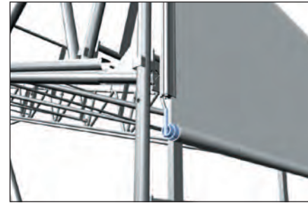
Tensioning using end pocket
