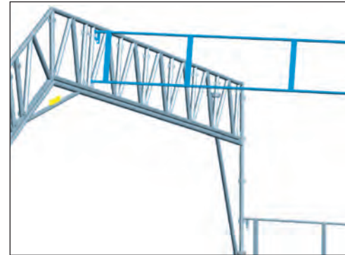
Figure 17 Working from the safety of the tower, locate Lacing frame into pockets on Ridge Frame, and level.
