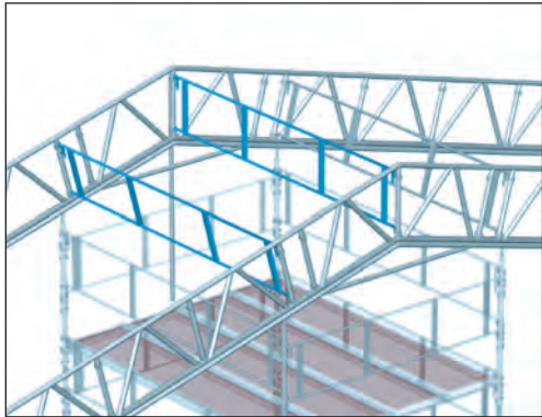
Figure 19 Fit additional 2 Lacing Frames to Ridge Frame.
